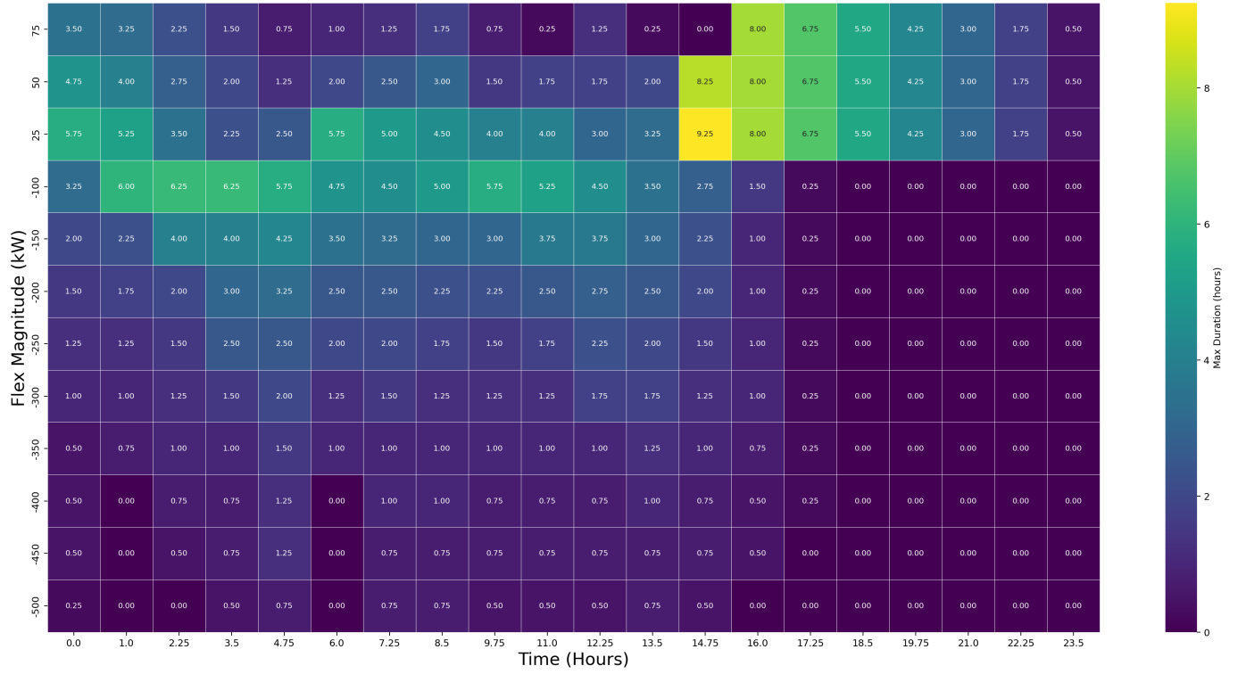
Fig. 7. Flexibility provision magnitude and duration. Cell values are the maximum feasible duration \tau in hours for each start time t_0 (x-axis) and requested power deviation \Delta P (y-axis). Positive \Delta P (top three rows) denotes downward flexibility (load increase) and negative \Delta P denotes upward flexibility (load reduction).
