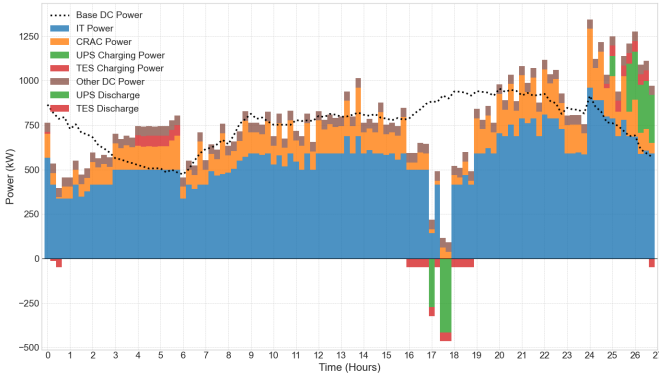
Fig. 6. Optimised DC Component Power Consumption
