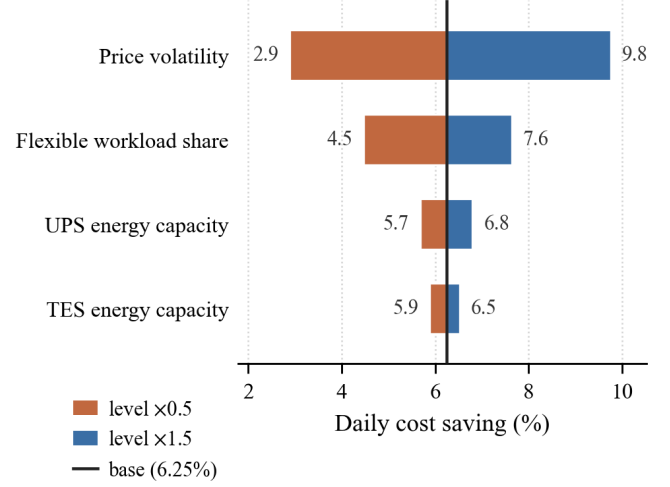
Fig. 10. Sensitivity of the daily cost saving to one-at-a-time parameter variations between 0.5\times and 1.5\times of the base value. The vertical line marks the base-case saving of 6.25%.
