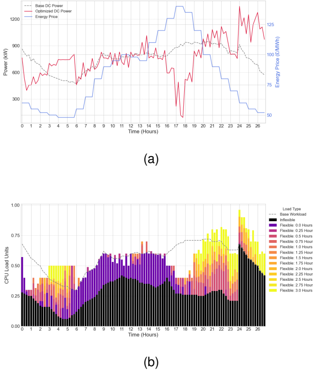
Fig. 5. (a) Power consumption profile and energy prices over the monitored period. (b) The corresponding IT workload distribution, shown as a stacked bar chart.
