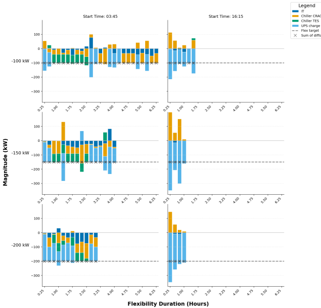
Fig. 8. DC component contributions to upward flexibility (negative \Delta P ). The six panels are arranged in a 3-by-2 grid: rows correspond to the requested flexibility magnitudes ( -100 , -150 and -200 kW, top to bottom) and columns to the start times (03:45, left; 16:15, right). Colours show the flexibility contribution of each DC asset.
