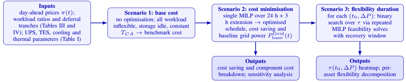
Fig. 4. Workflow of the three-scenario optimisation and flexibility assessment. Scenario 1 provides the unoptimised cost benchmark, Scenario 2 establishes the cost-optimised baseline, and Scenario 3 quantifies the maximum feasible flexibility duration for each requested start time and power deviation while enforcing recovery.
